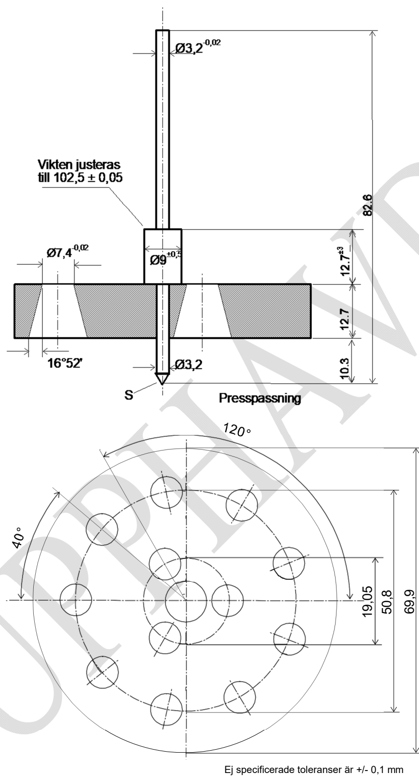
Figur 1: Penetrometer
